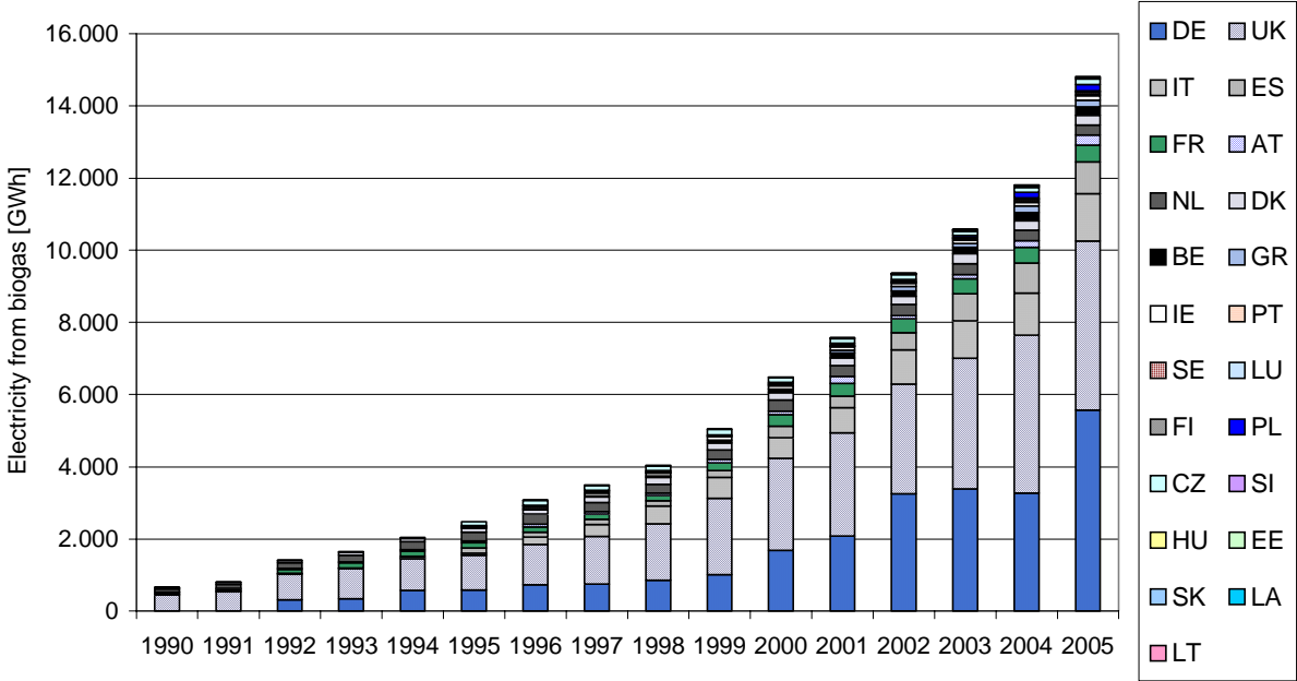
Figure 8: Historical development of electricity generation from biogas in the EU-25 Member States from 1990 to 2005 27 .
